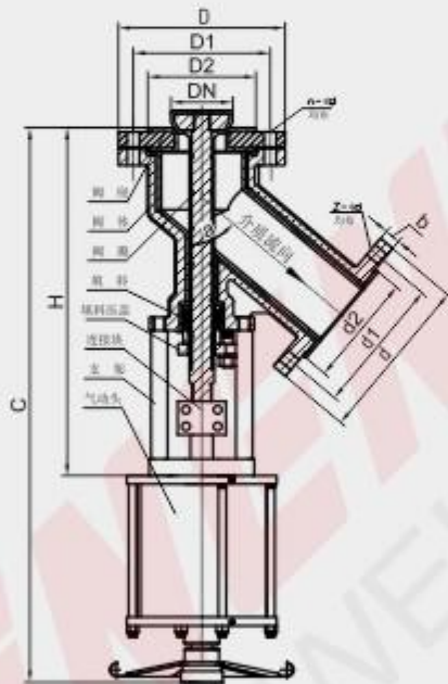
FLJ641PFA/F46/F4-16
