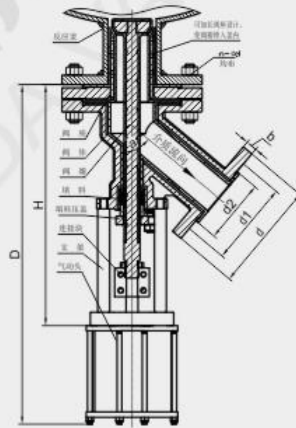
FLJ641PFA/F46/F4-16
