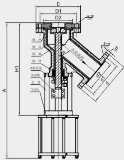
FLJ642PFA/F46/F4-16
